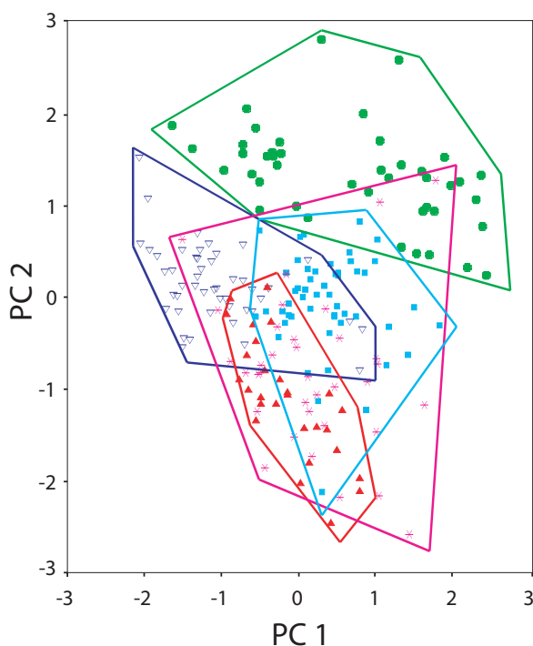
Fig. 3: Scatter plot of scores resulting from Principal Components Analysis with continuous characters representing Trochosa females on the two components axes (PC 1-2). te = Trochosa terricola ; sp = T. spinipalpis ; ru = T. ruricola ; ro = T. robusta ; hi = T. hispanica .
