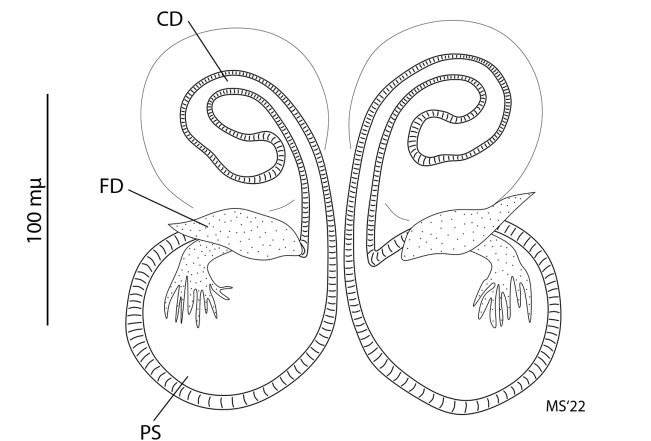
Abb. 13: Euophrys canariensis , Weibchen von Teneriffa, Vulva dorsal Fig. 13: Euophrys canariensis , female from Tenerife, vulva dorsal view
